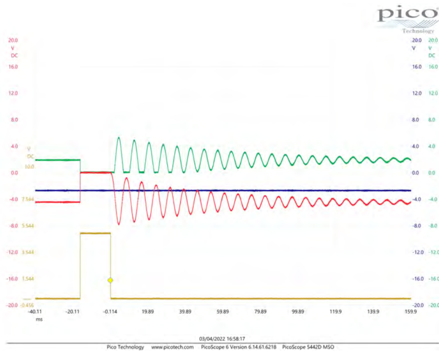
Figure 6: Bungee cord behaviour
