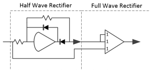
Figure 4: Ideal rectifiers
