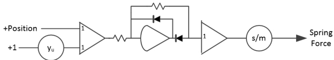
Figure 5: Bungee cord model
