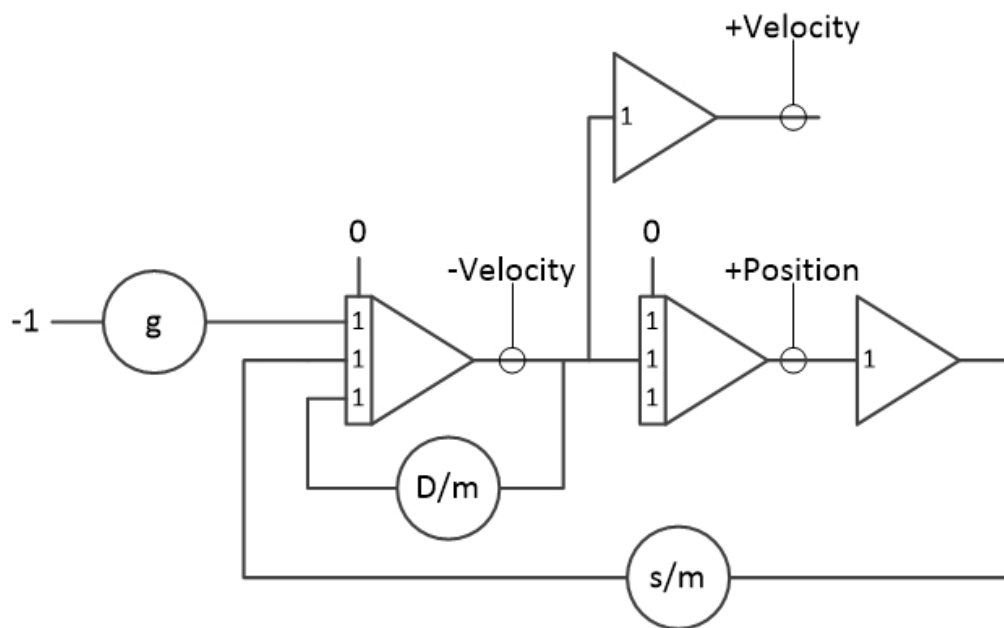
Figure 2: Setup for the spring-mass-damper problem
