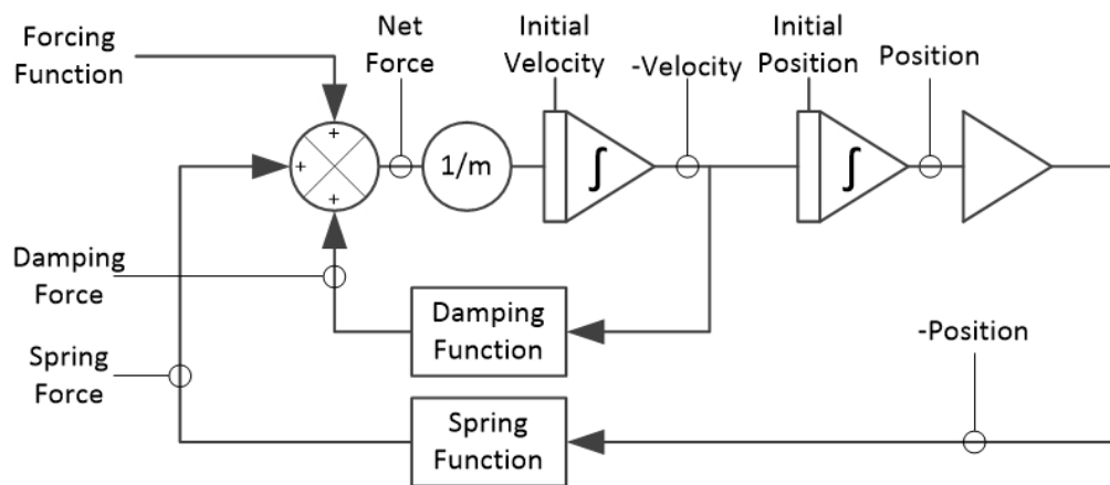
Figure 1: Generalized spring-mass-damper problem
