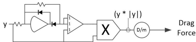
Figure 7: Aerodynamic drag model
