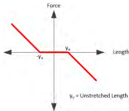
Figure 3: Force vs. length for bungee cord
